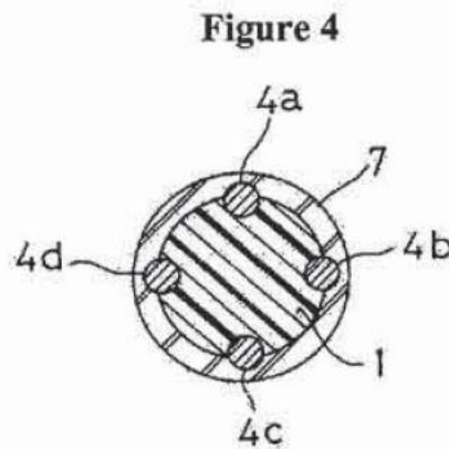
Figure 4 shows a cross-section of the finished cable
