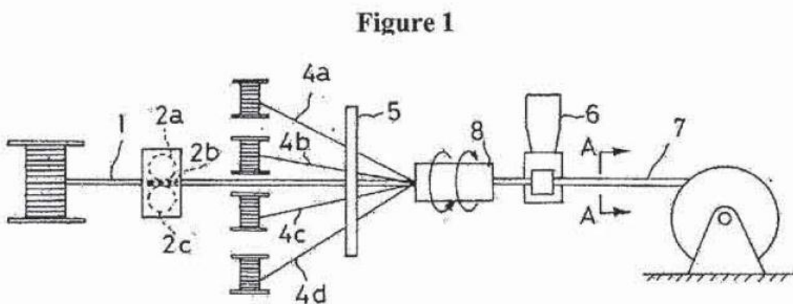
Figure 1 illustrates an assembly for carrying out the method of forming a cable disclosed in JP '910
