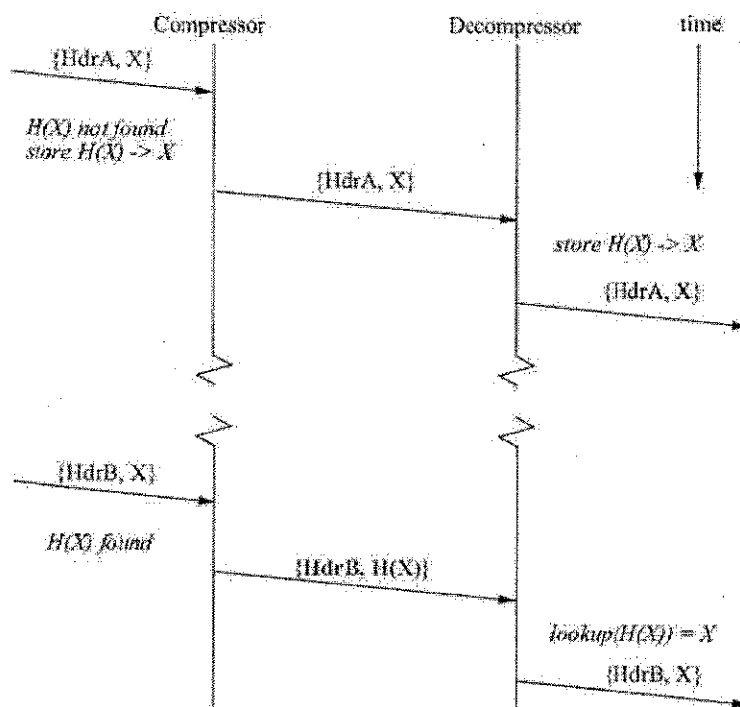
Figure 4: Compression protocol
