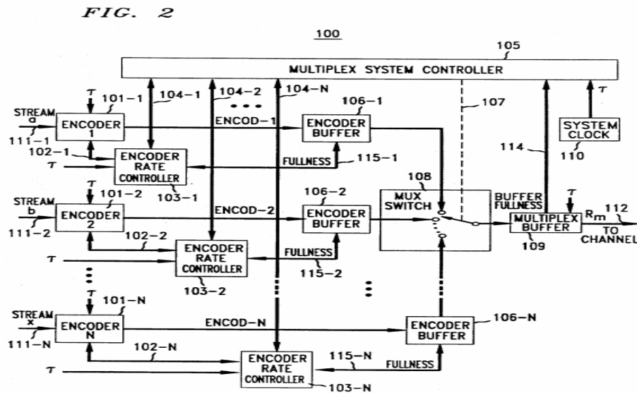
Figure 2 illustrates encoding system 100 wherein a number of individual unencoded bit streams 111-1 through 111-N are encoded and multiplexed into a single bit-stream 112 for transmission.
