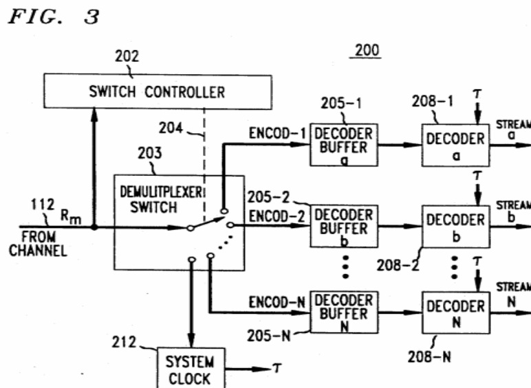
Figure 3 illustrates a demultiplexer and decoder system 200 that corresponds to the encoding system 100 illustrated in Figure 2.
